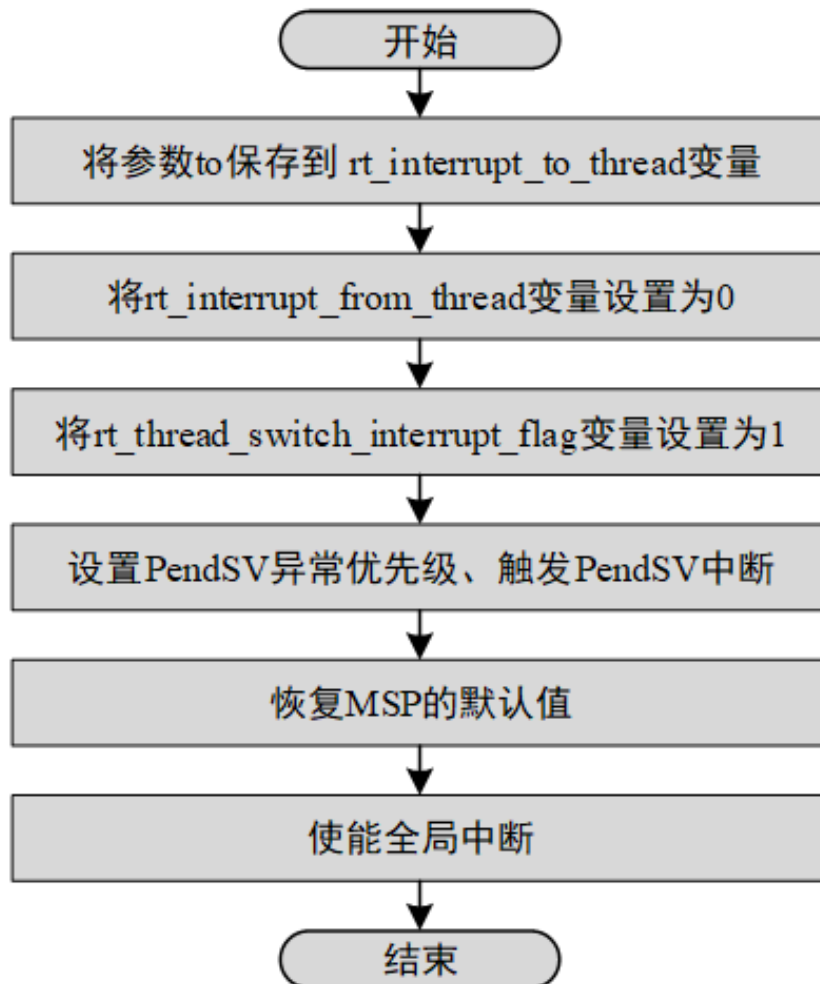
图 9.4: rt_hw_context_switch_to() 流程图
