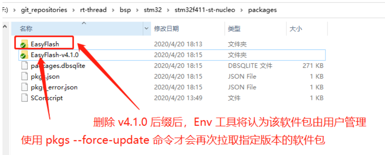
图 10.10: user_manage_package
