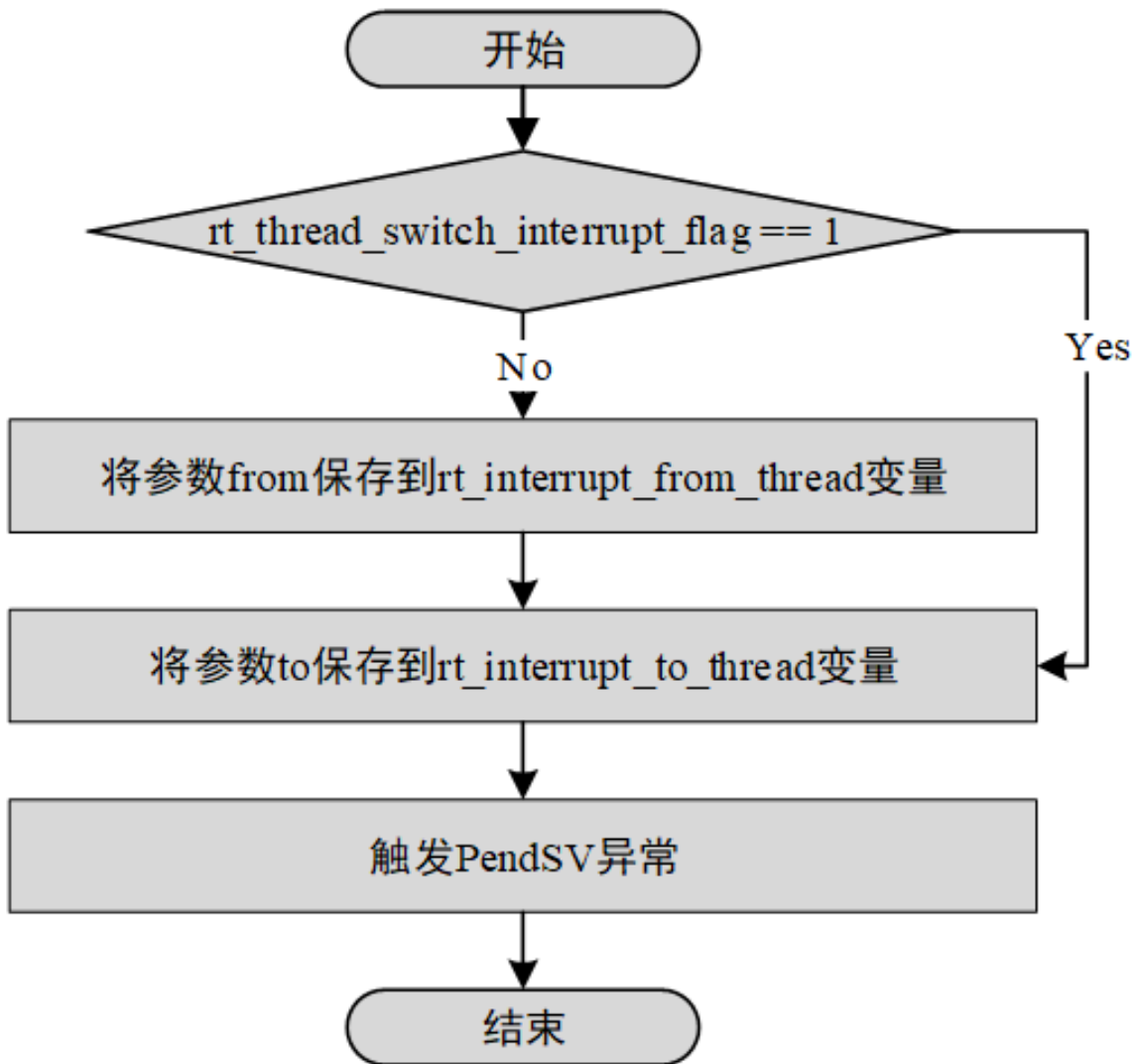
图 9.5: rt_hw_context_switch()/rt_hw_context_switch_interrupt() 流程图
