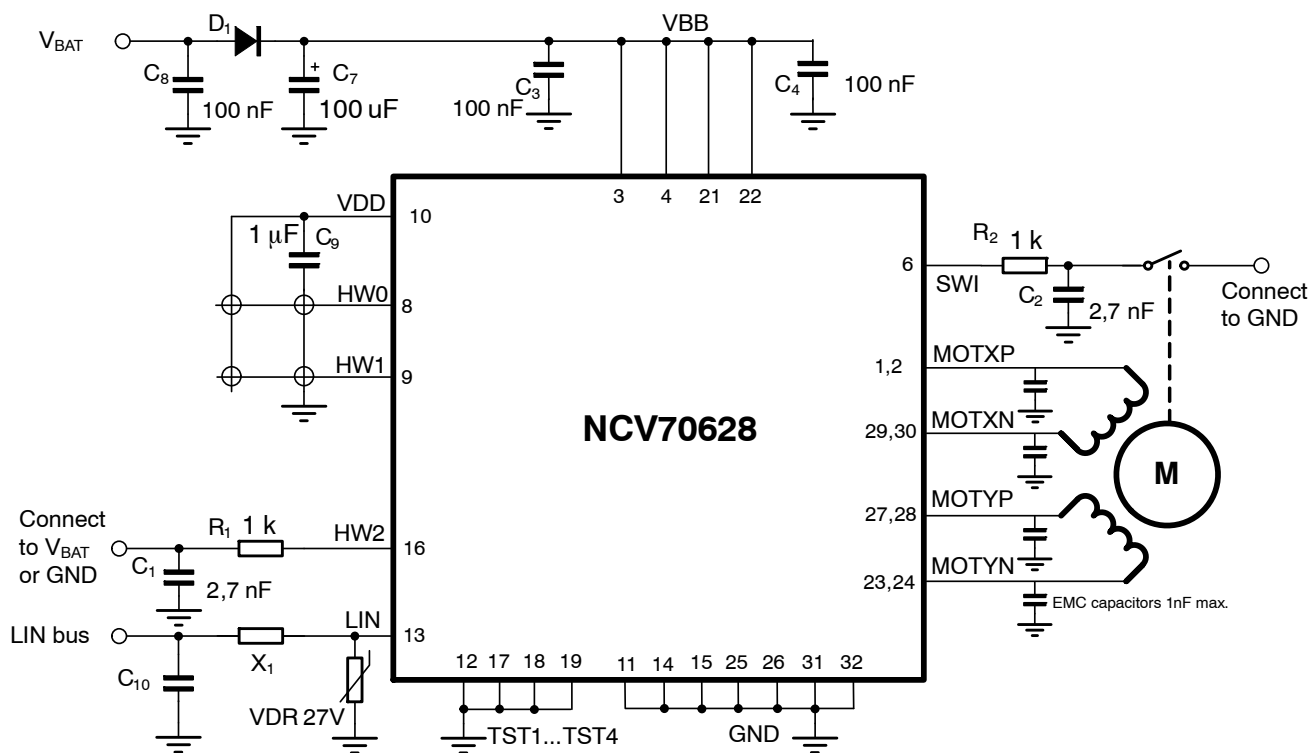
Figure 5. Typical Application
