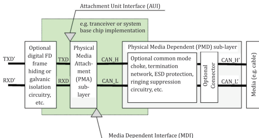
Figure A.1 — Optional functions in this document, compliant transceiver and their relation to the OSI sublayers
