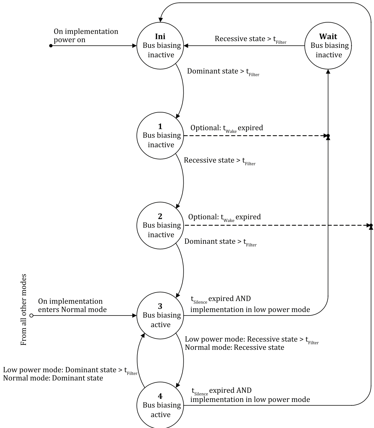
Figure 11 — Bus biasing control for automatic voltage biasing
