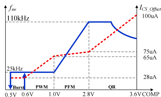
Fig. 1 Frequency & Ipk Modulation
