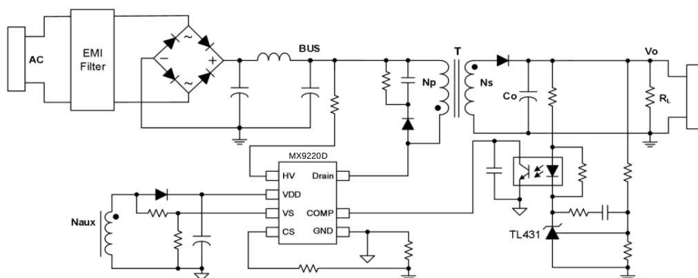
MX9220D Typical Application
