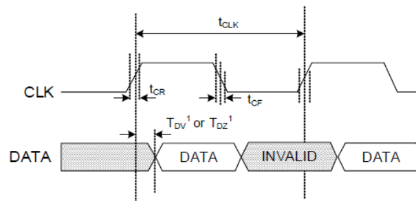
Figure 17. PDM Timing - SDR Mode
