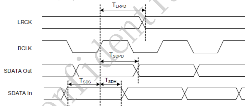
Figure 13. I2S Master Mode Timing
