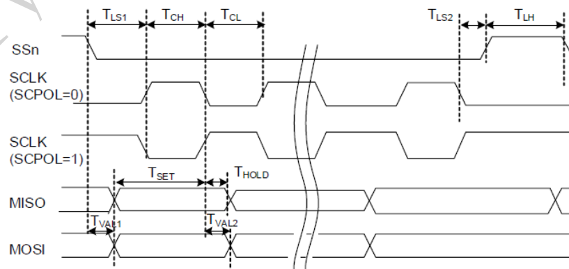
Figure 10. Motorola SPI Mode 1/3 (SCPH = 1)
