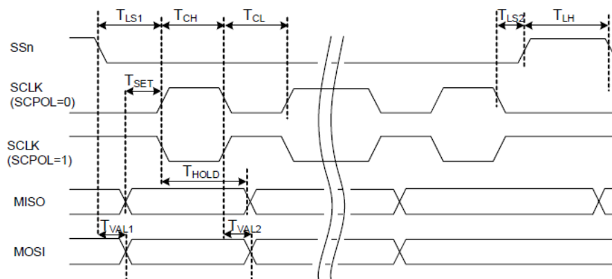
Figure 9. Motorola SPI Mode 0/2 (SCPH = 0)
