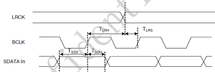
Figure 14. I2S Slave Mode Timing
