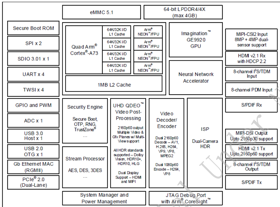
Figure 1. SN3680(VS680) High-level block diagram
