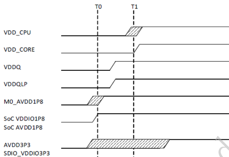
Figure 4. SN3680(VS680) Recommended power-up sequence in SoC power domain
