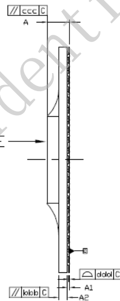
Figure 20. SN3680(VS680) Side View
