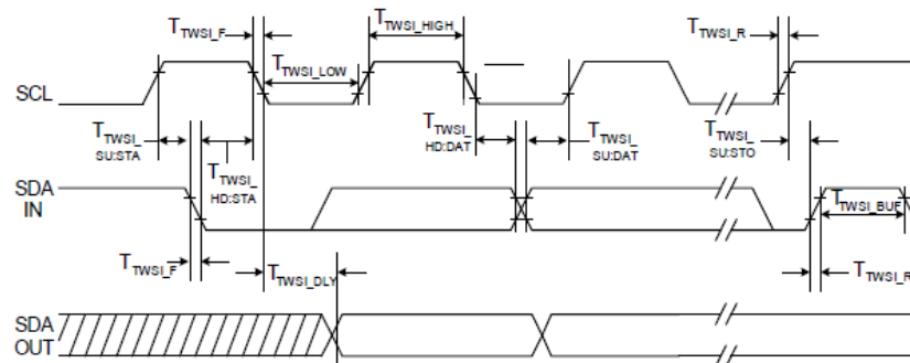
Figure 7. Two-Wire Serial Interface Timing
