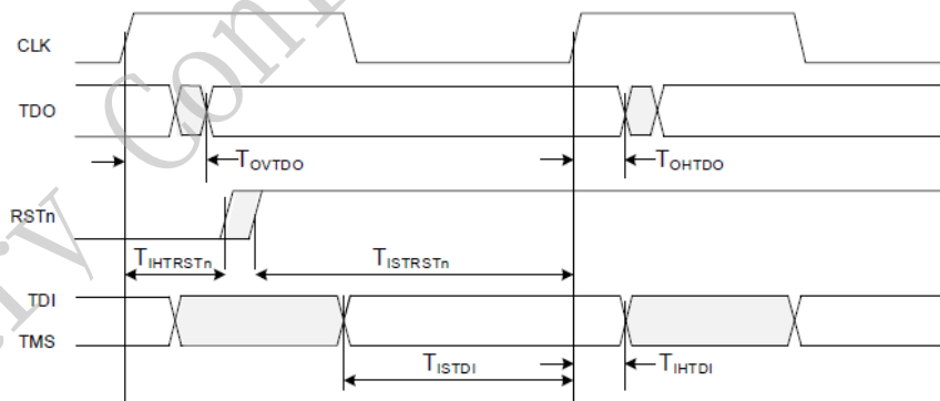
Figure 11. JTAG Timing
