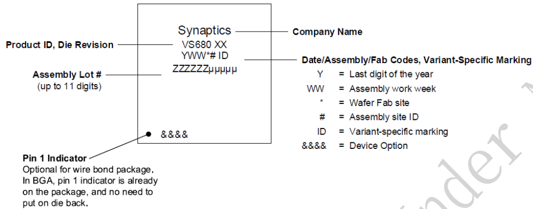
Figure 22. Commercial Package Marking and Pin 1 Location
