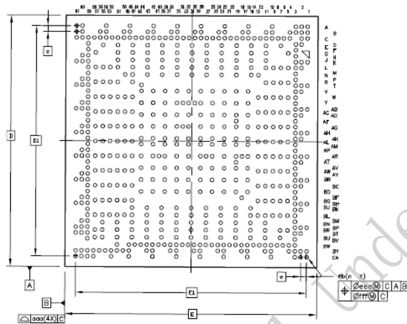
Figure 21. SN3680(VS680) Bottom View
