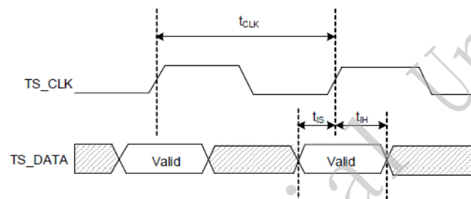
Figure 12. Transport Stream Serial Input Timing
