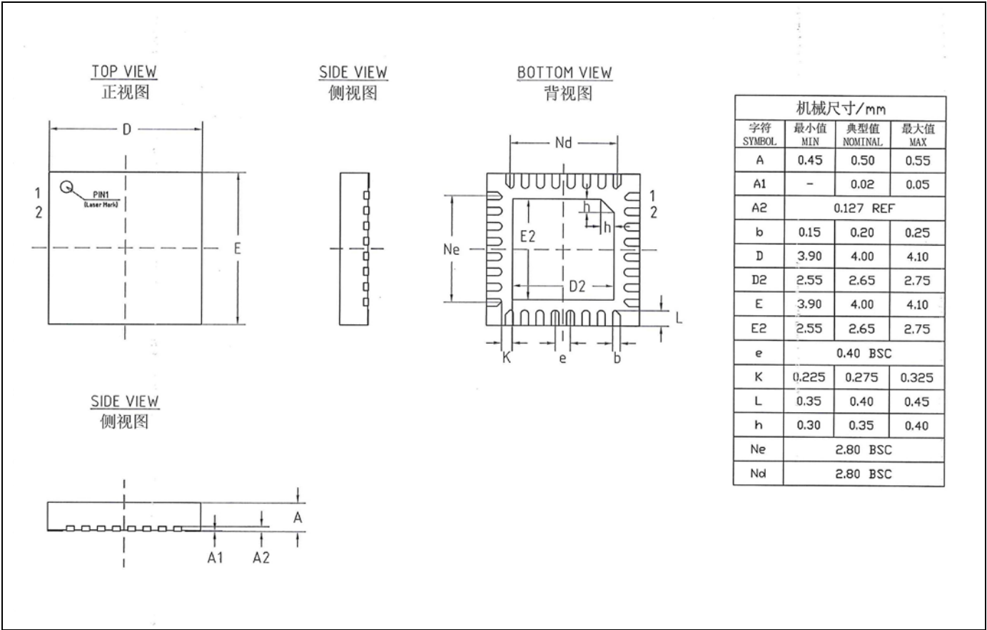
Figure 4-4 QFN32 (4x4-P0.4mm)封装尺寸
