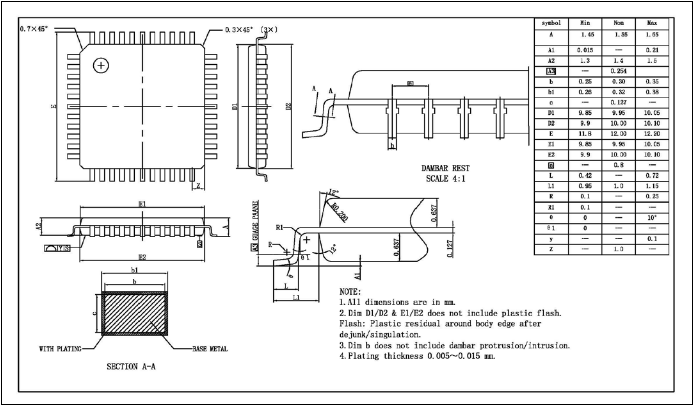
Figure 4-2 44-QFP (10x10-P0.8mm) 封装尺寸
