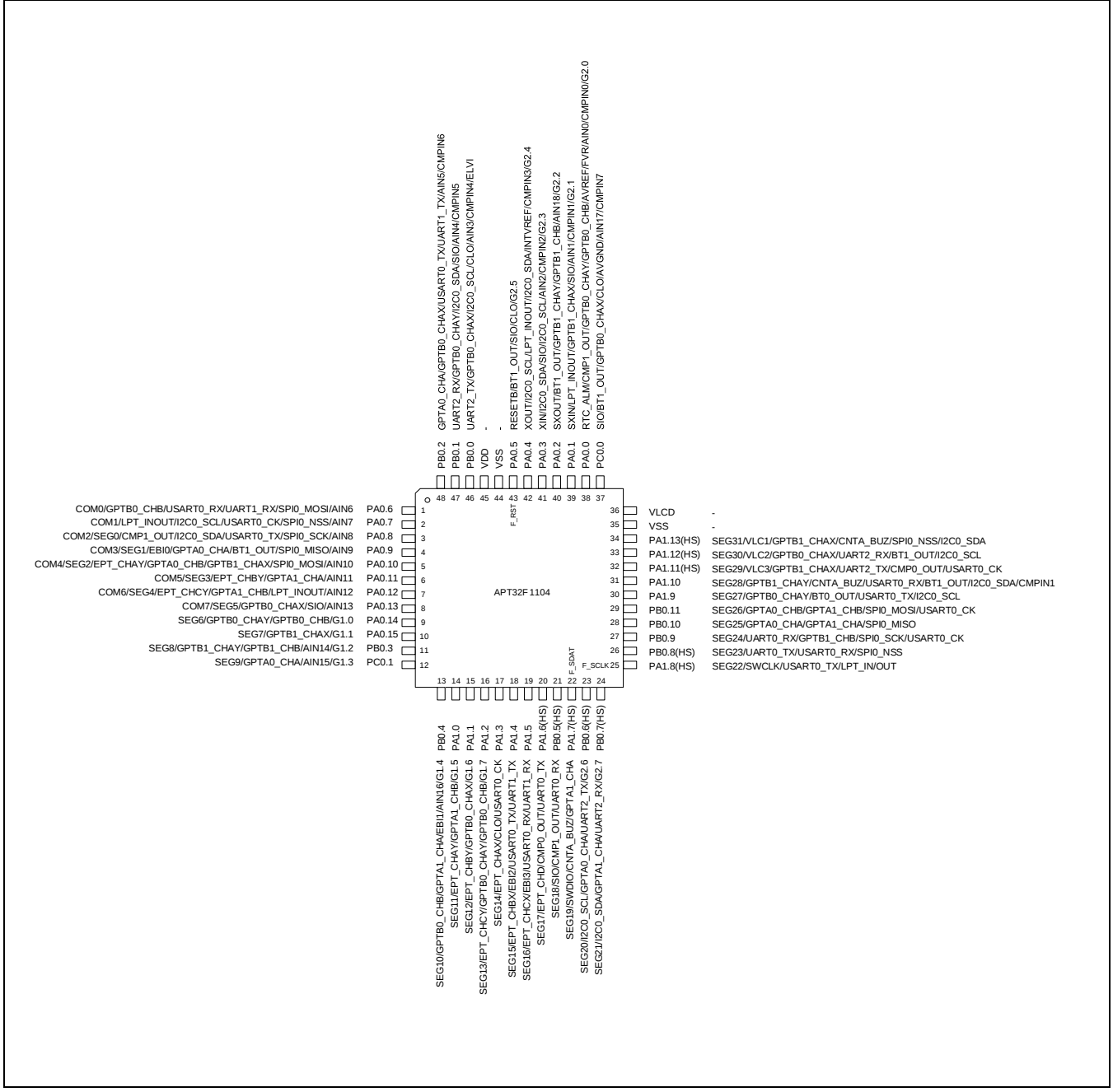
Figure 2-1 管脚定义图(48 LQFP)
