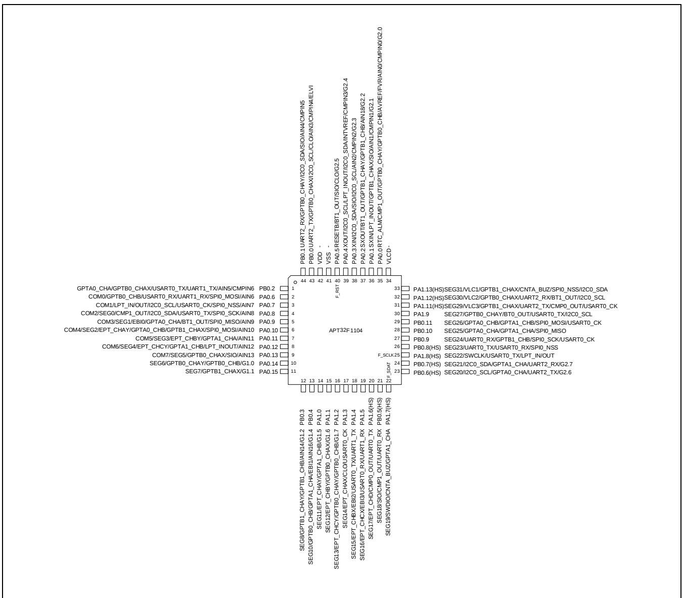
Figure 2-2 管脚定义图(44 QFP)
