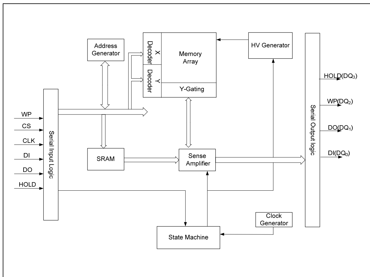
Figure 1 FM25Q08 Serial Flash Memory Block Diagram
