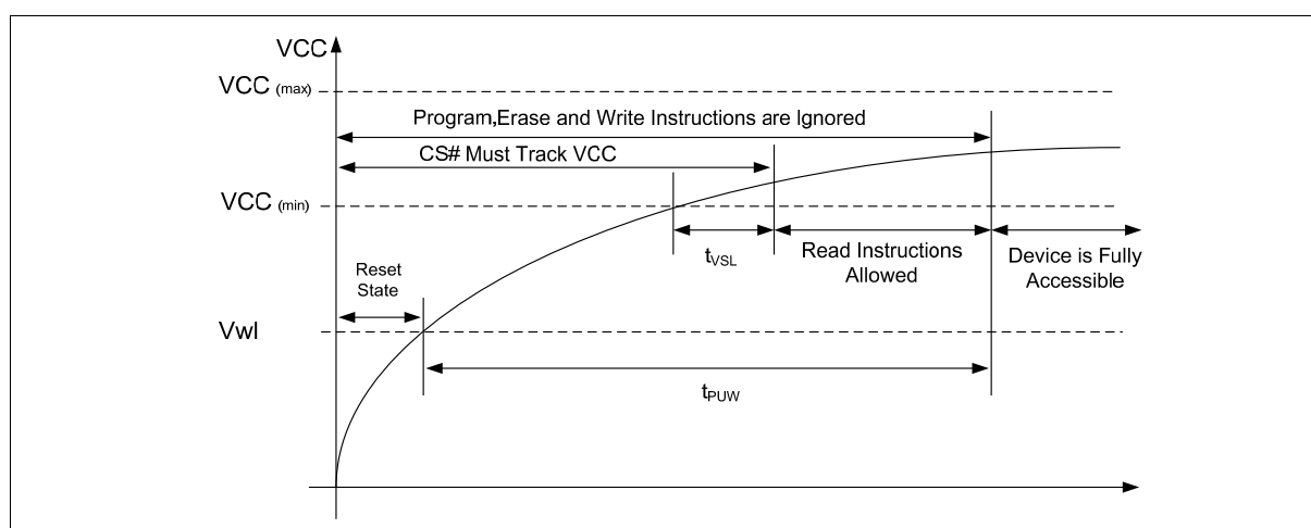
Figure 66 Power-up Timing
