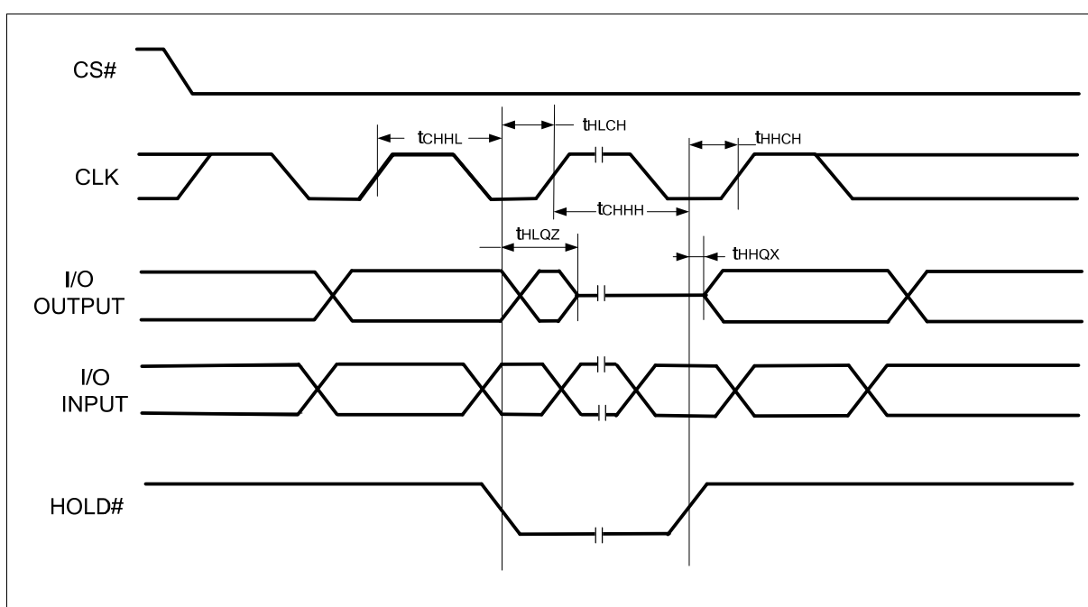
Figure 70 Hold Timing
