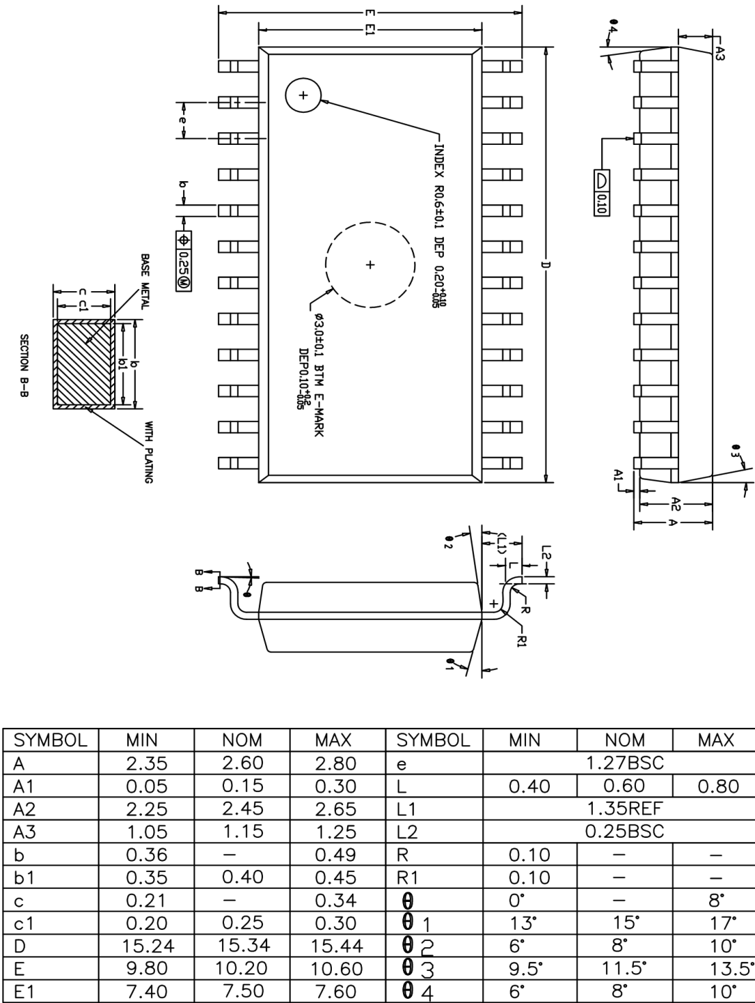
Figure 4-2 SOP24 (1.27mm)封装尺寸
