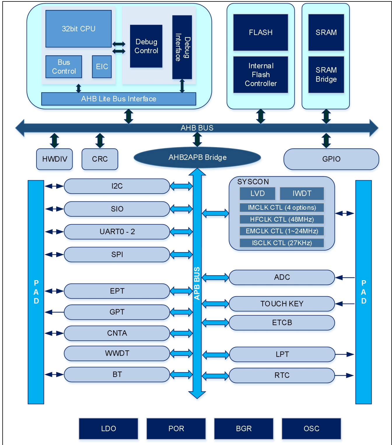
Figure 1-1 APT32S1028模块框图
