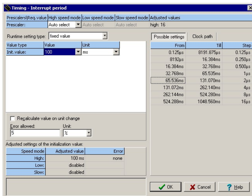
Figure 1.4 - Timing dialog box allows a user friendly setting of components' timing
