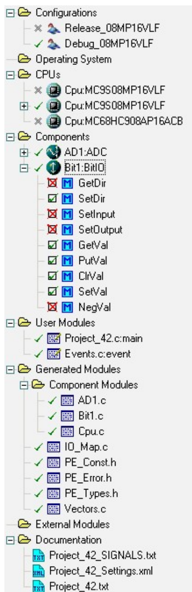
Figure 2.5 - The content of the Project Panel
