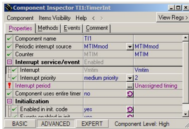
Figure 2.27 - Component Inspector Window
