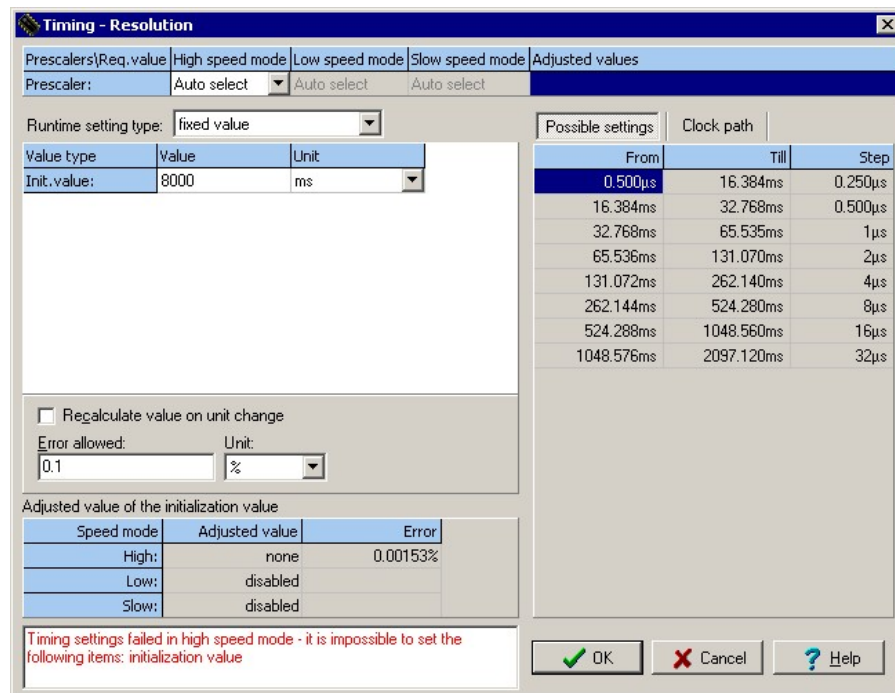
Figure 2.28 - Timing Settings Dialog
