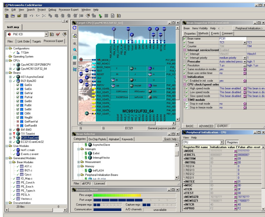
Figure 1.1 - CodeWarrior IDE with Processor Expert active
