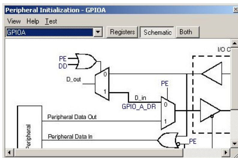
Figure 2.48 - Schematic Diagram of the Peripheral
