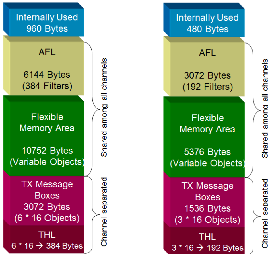
Figure 1.2 Memory Layout of RS-CANFD V2: 6-channel, 3-channel versions
