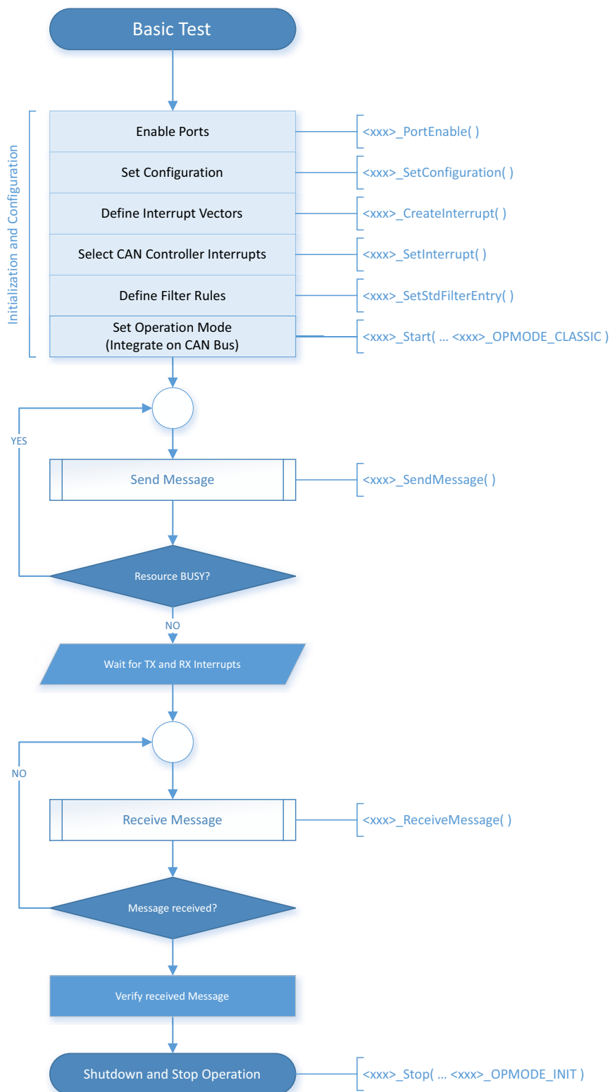
Figure 5.5 M_(TT)CAN Basic Communication Application Example
