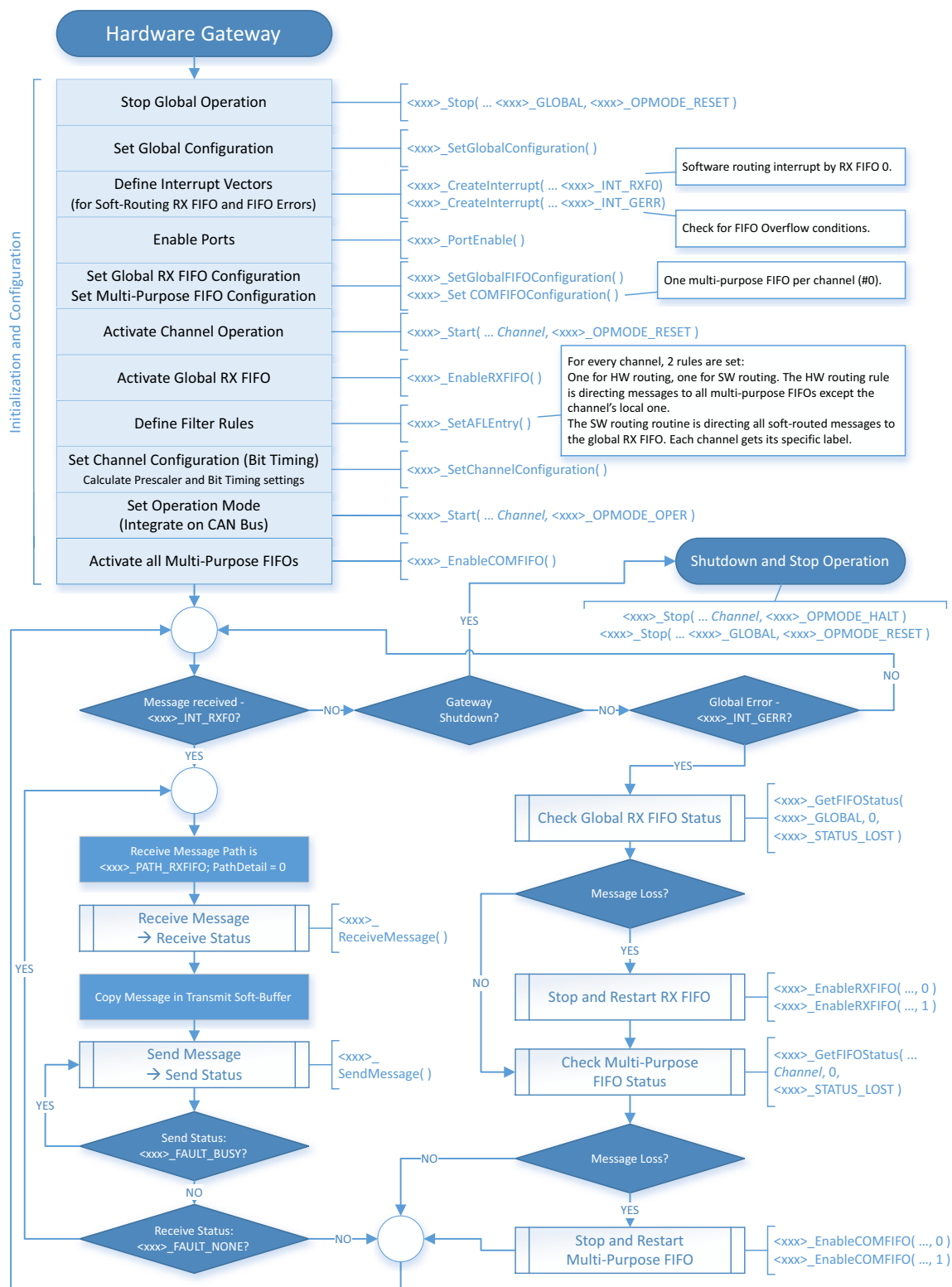
Figure 5.7 RS-CAN(-FD) Hardware-Gateway Application Example
