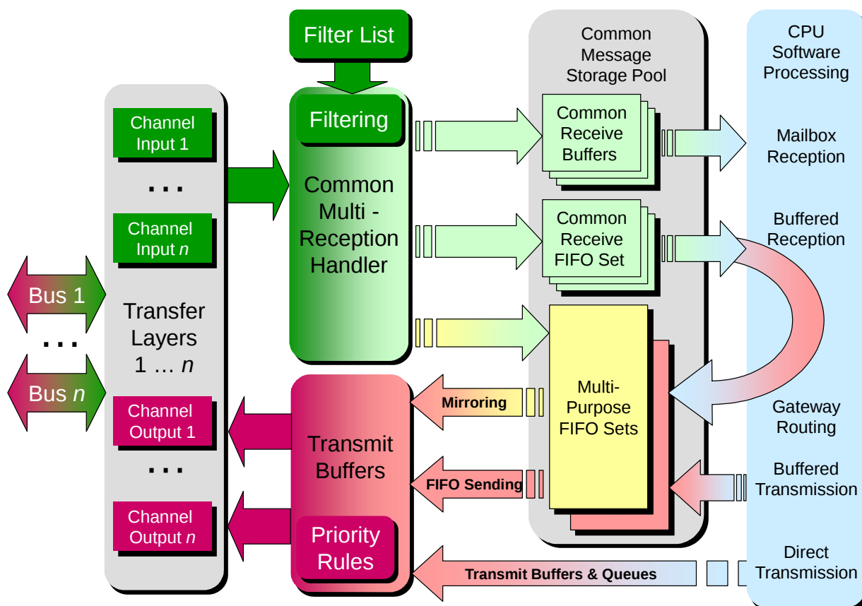
Figure 1.1 State of the art CAN Controller RS-CANFD
