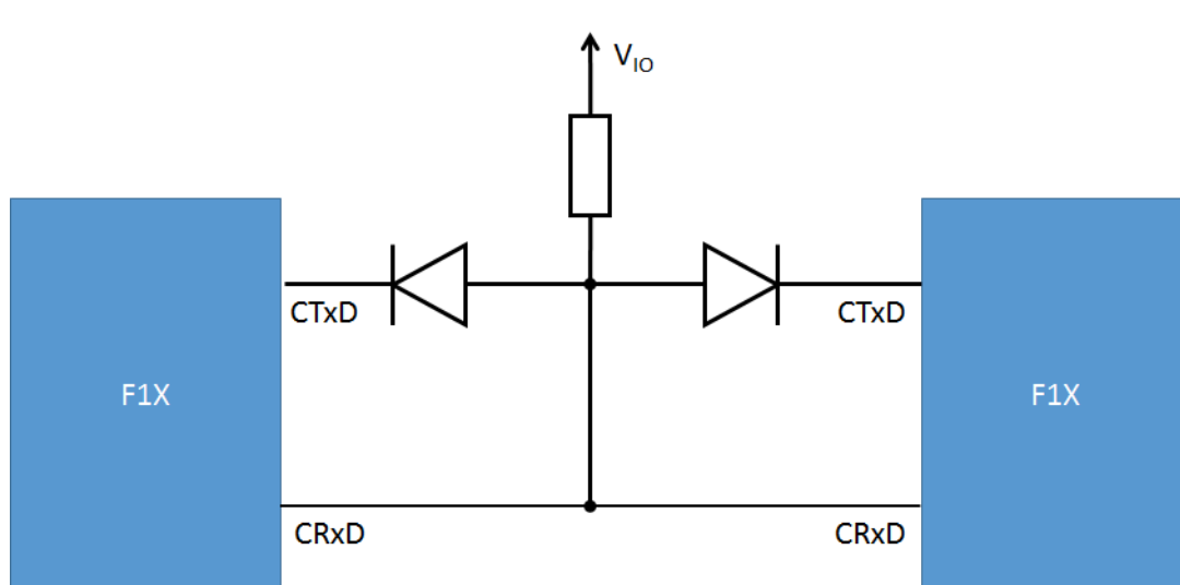
Figure 2.1 CAN Bus without Transceivers
