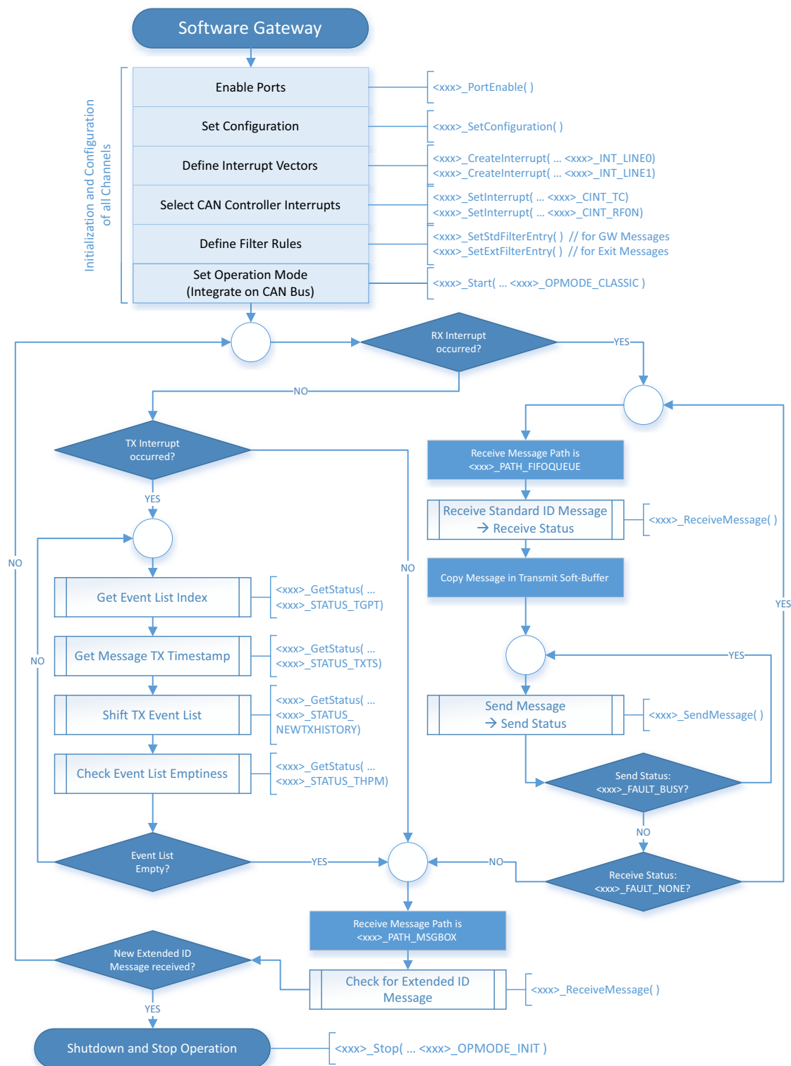
Figure 5.6 M_(TT)CAN Soft-Gateway Application Example
