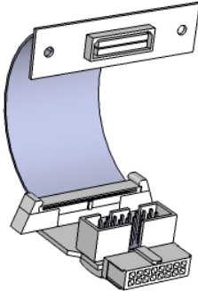
Active pod (JTAG COP and ColdFire targets) ‡
